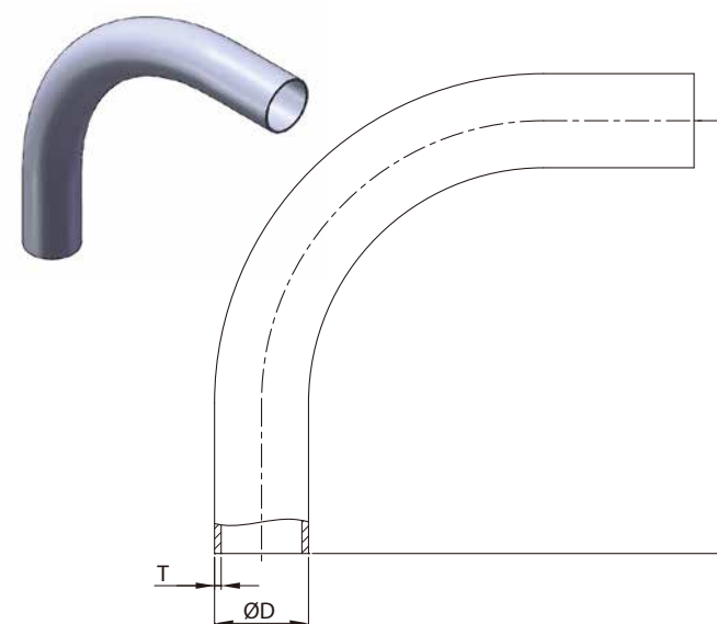
LONG 90° ELBOW (3D)
